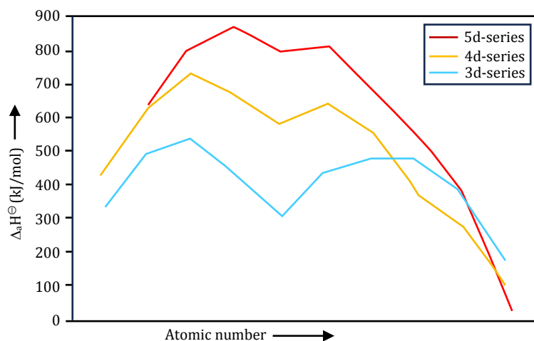
Trends in enthalpies of atomization of transition elements
