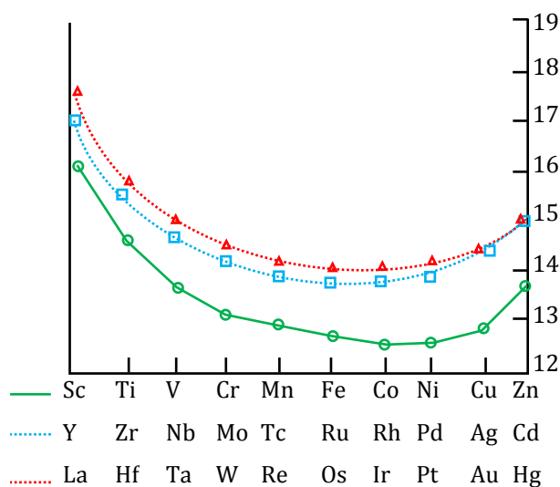
Trends in atomic radii of transition elements
