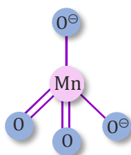
Tetrahedral manganate (green) ion
